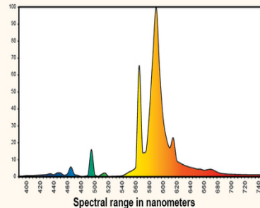
High Pressure Sodium Dimmed 50% (results in lamp output of only 40%)
