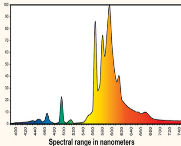
High Pressure Sodium Operating @ 75% (results in lamp output of only 70%)
