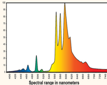
High Pressure Sodium Operating @ 100% (results in 100% output)
